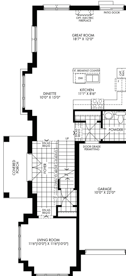
MAIN A
