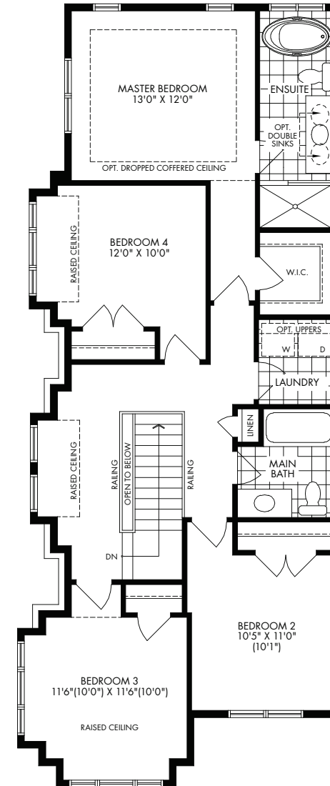
UPPER A
